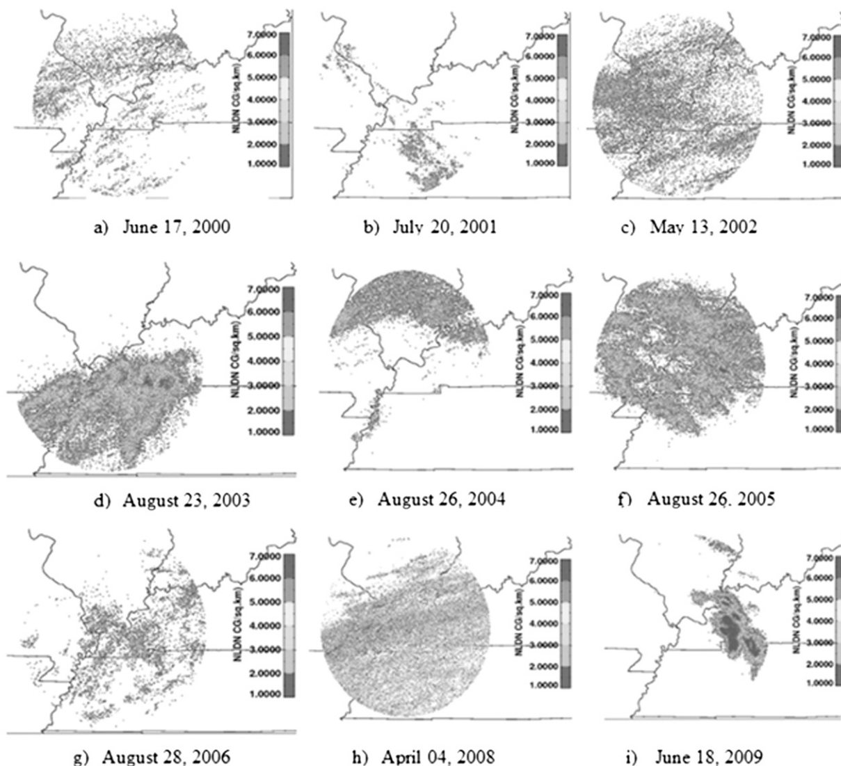
FIG. 6. NLDN C-G lightning density (strikes \text{km}^{-2} ) for the KPAH site horizontal swath coverage.
