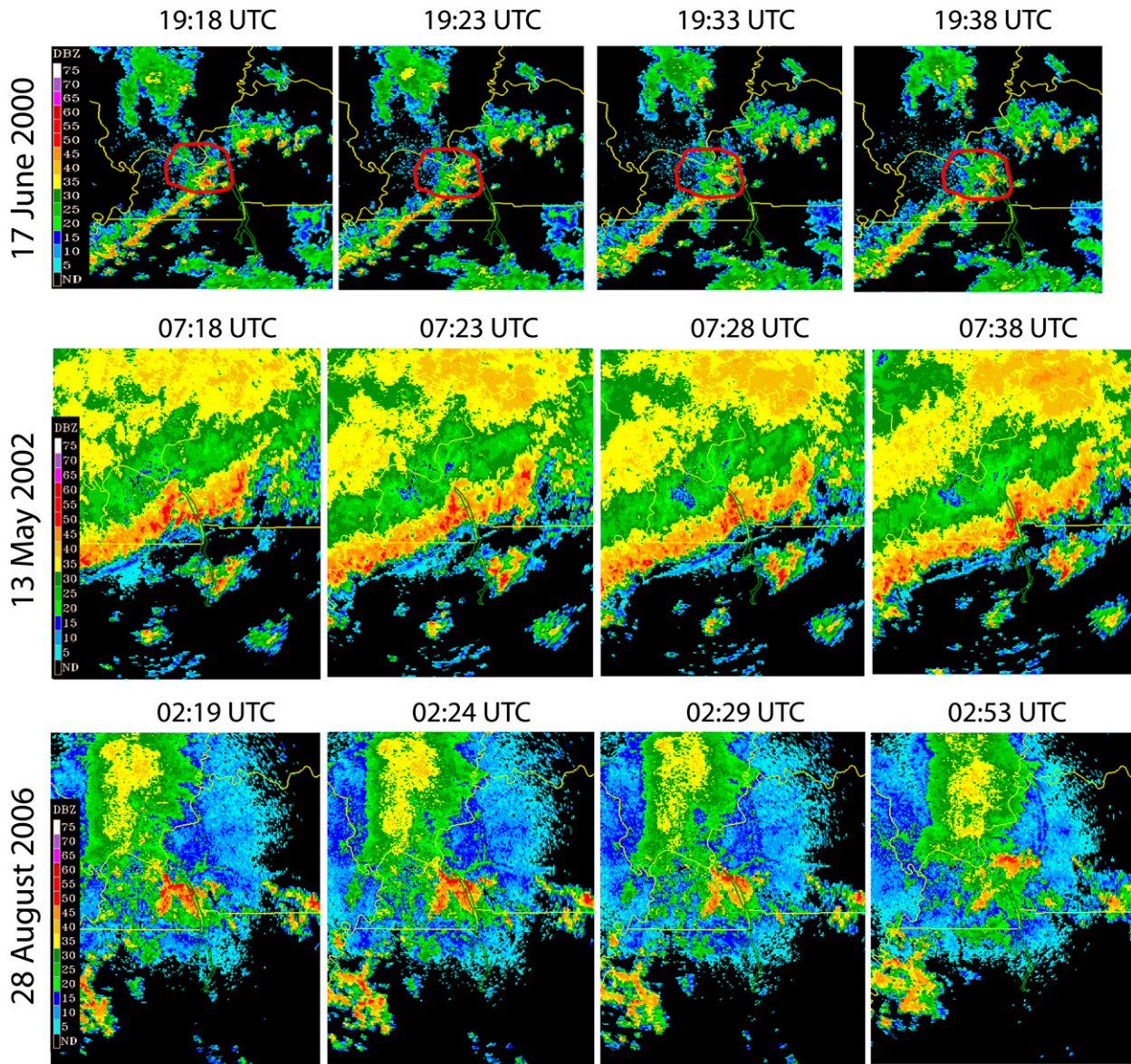
FIG. 7. Time evolution of NEXRAD radar imagery for selected events (category I).
