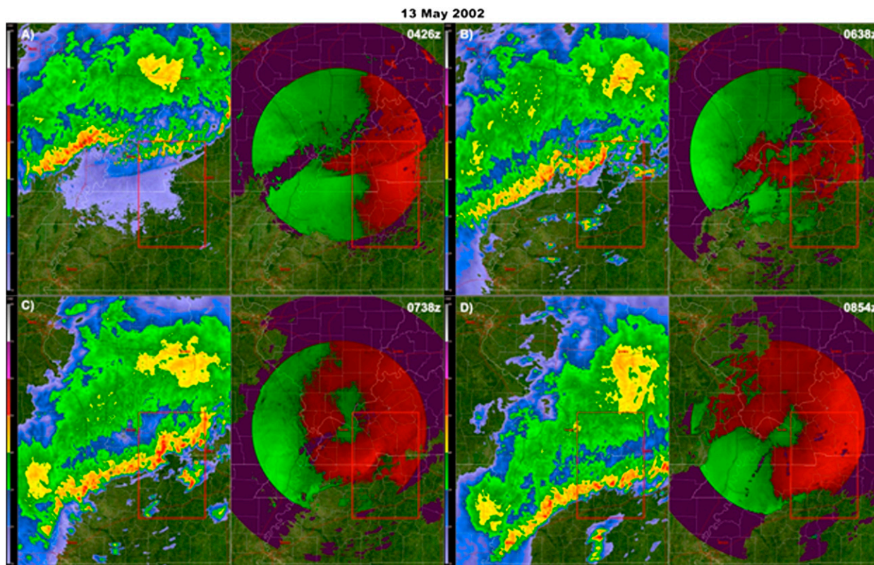
FIG. 10. For each letter-labeled panel (a)–(d), base (left) reflectivity and (right) velocity from the KPAH site during 13 May 2002 (category I): (a) 0426, (b) 0638, (c) 0738, and (d) 0854 UTC. The red box in each panel denotes the LBL domain.
